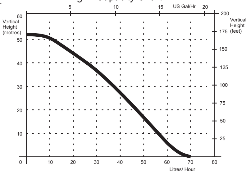
fig.2 Capacity Chart
